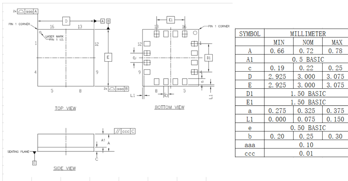
Figure 5. Package Size
