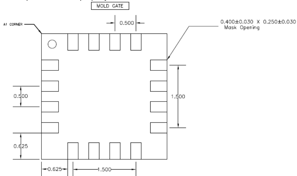
Figure 7. QMC5883P PCB footprint
