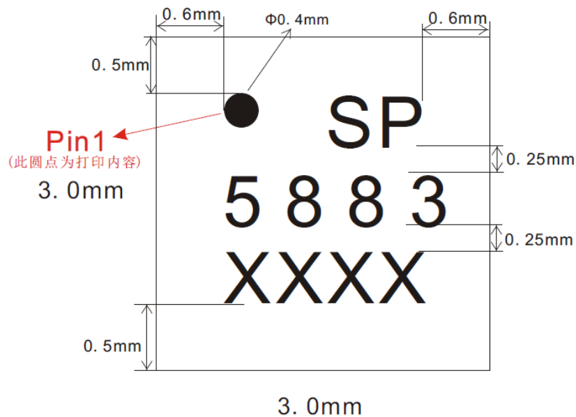
Figure 4. Chip Marking
